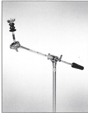
B78 2-piece hideaway boom cymbal arm (20.1-inch) with 2.2 lb counterweight, universal ball-in-socket tilter, knurled boom arm and OS Cymbal Accentuator
