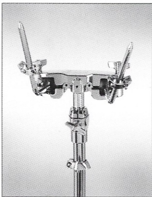
TH675 Tom shaft and arm set for Pro M Series Tube Diameter: 25mm
