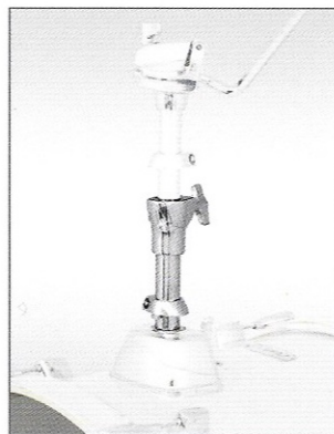
6705-075A Tube expander allows TH684 Single Tom Arm (22mm) to fit into standard size bass drum tom holder receiver (25mm).
